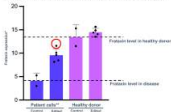
5 different dual-flap Prime Editors all restore frataxin expression levels in patient cells toward levels in healthy donor cells
